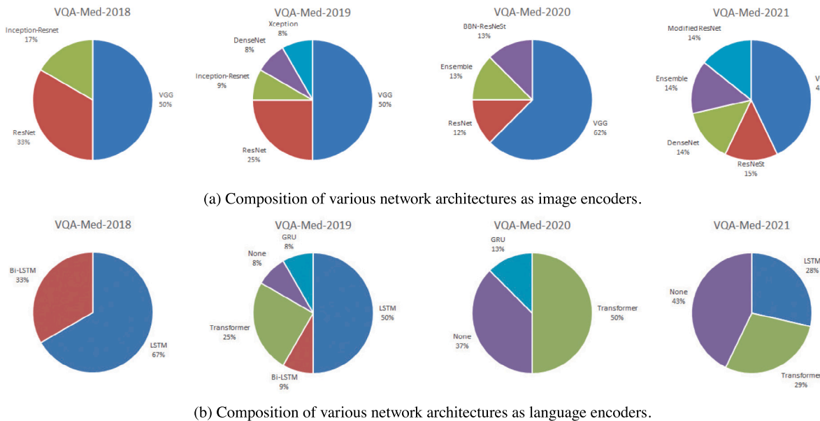
Fig. 4. The encoders used in VQA-Med challenges.
