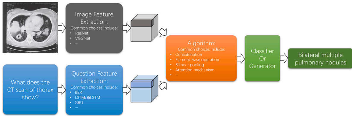
Fig. 3. A schematic diagram of the mainstream medical VQA frameworks illustrating main components, including image feature extraction, question feature extraction, feature fusion, and answering component.
